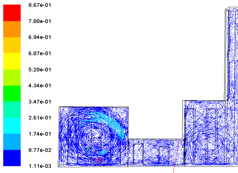
Fig. 4. Air movement in the plane of z = 3 m.
