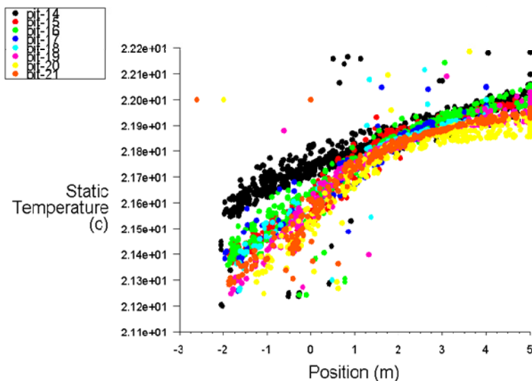
Fig. 7. Relationships between temperature and position for all 8 pits in 8 chosen planes in the range of 21.2°C to 22.2°C.
