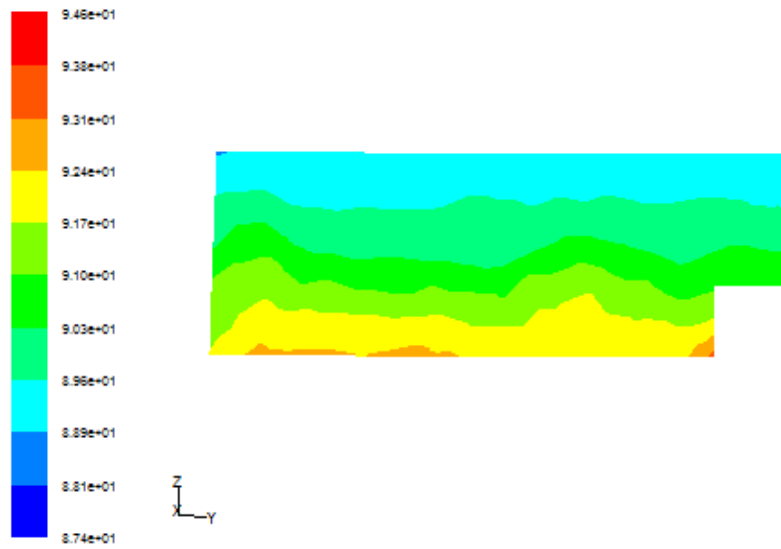
Fig. 8. RH distribution for pit 16.
