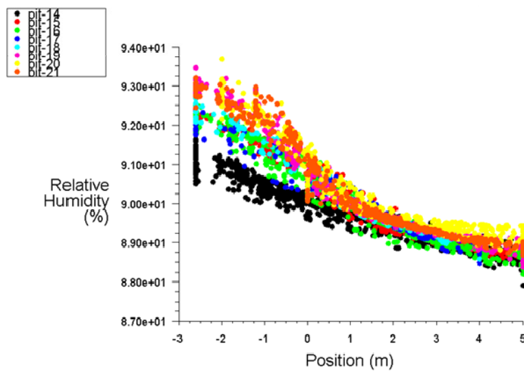
Fig. 10. Relationships between RH and position in z direction for all 8 pits in 8 chosen planes.
