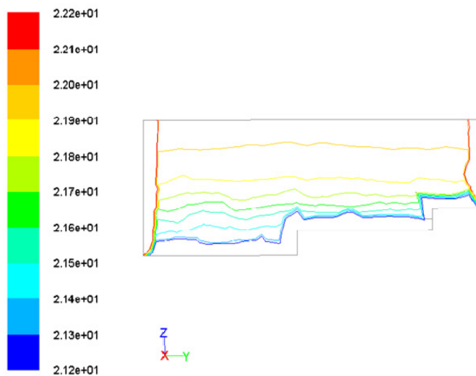
Fig. 5. Temperature distribution in plane x = 3.9 m for pit 21.
