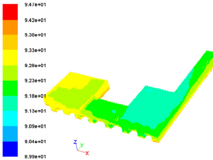
Fig. 11. Overall RH distribution in the suggestion program.
