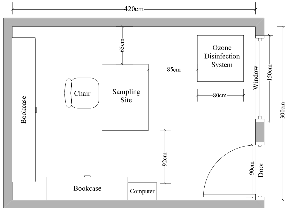
Fig. 2. Layout of ozone disinfection system in office.
