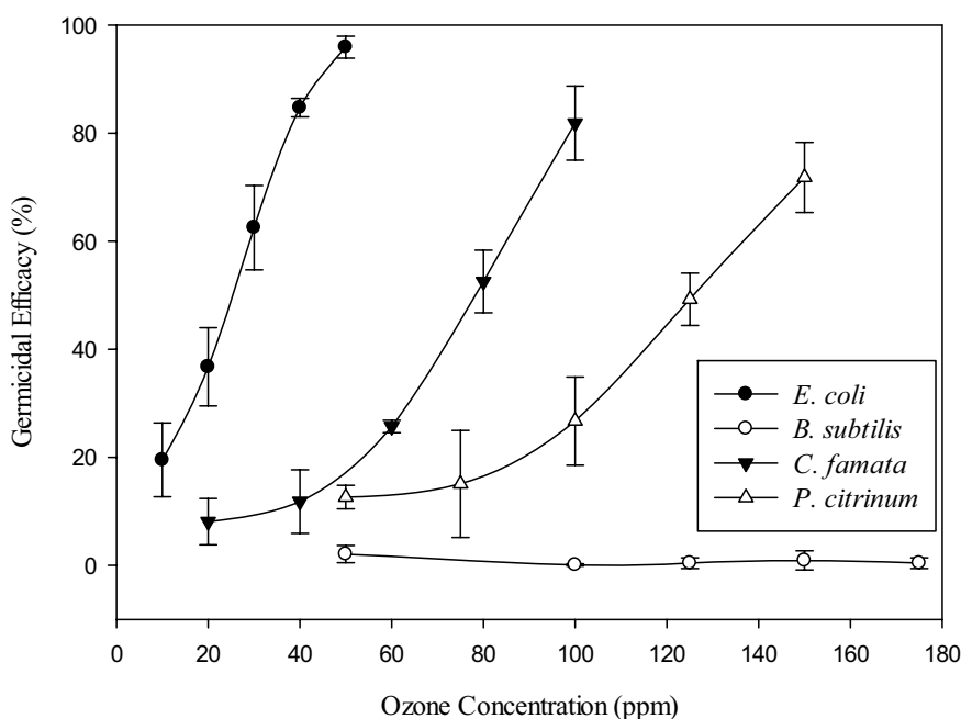
Fig. 3. The germicidal efficacy of ozone on bioaerosols at an RH of 50% and retention time of 10 s.
