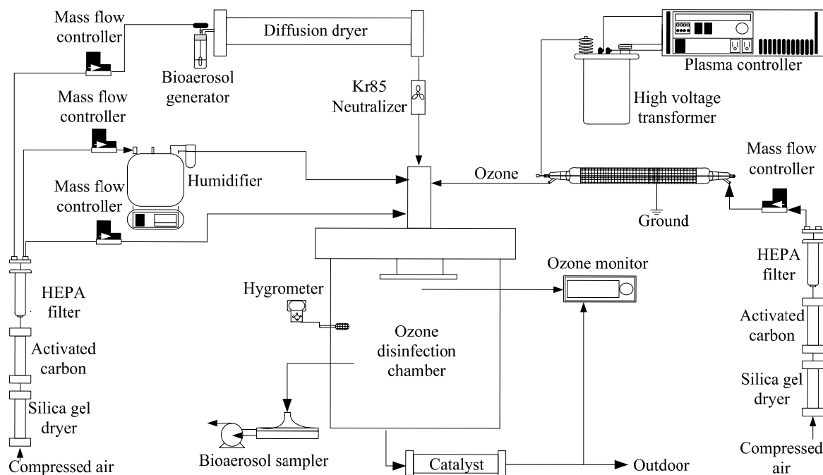
Fig. 1. Ozone disinfection system for bioaerosols.
