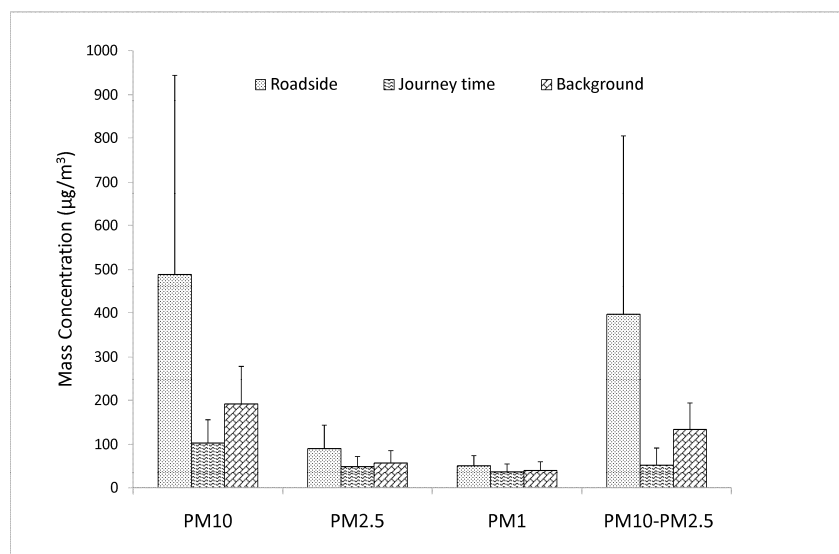
Fig. 2. Overall roadside, journey time and background levels of PM 10 , PM 2.5 PM 1 (µg/m 3 ) in Lahore.
