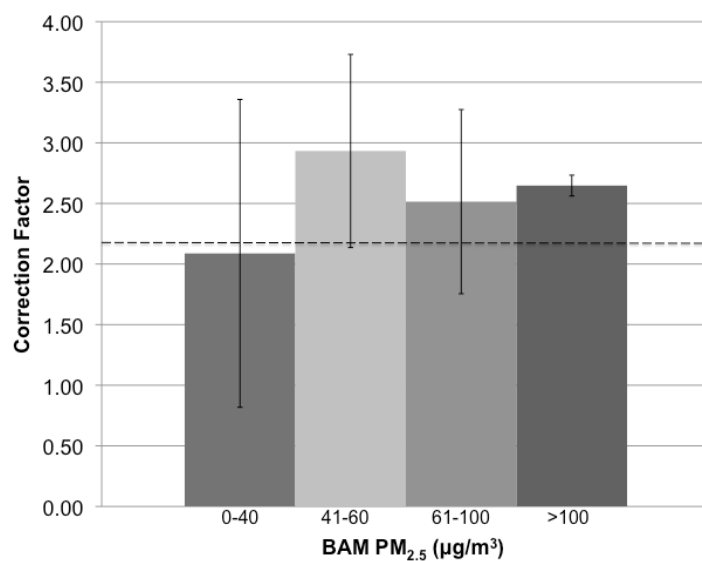
Fig. 2. Average correction factor values \pm standard deviation under laboratory conditions at concentration ranges of 0–40, 41–60, 61–100, and >100 \mu\text{g}/\text{m}^3 PM_{2.5} ( n = 79, 6, 3, 2 , respectively). One-way ANOVA p = 0.34 . Dashed line indicates overall average of 2.18.
