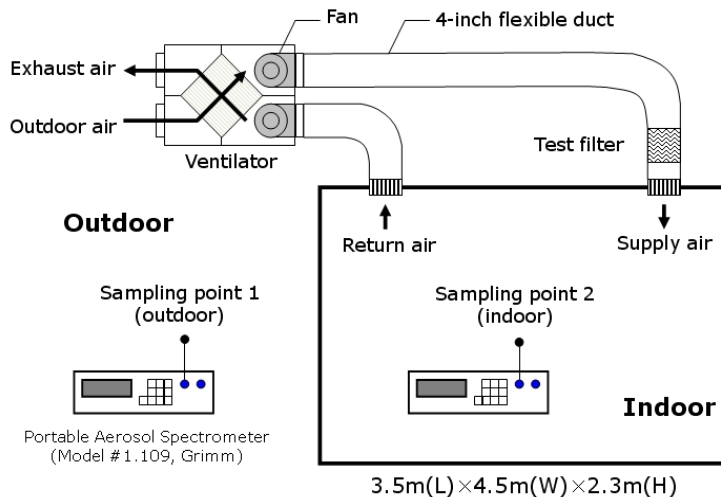
Fig. 5. Schematic of the room and ventilation apparatuses for field tests.
