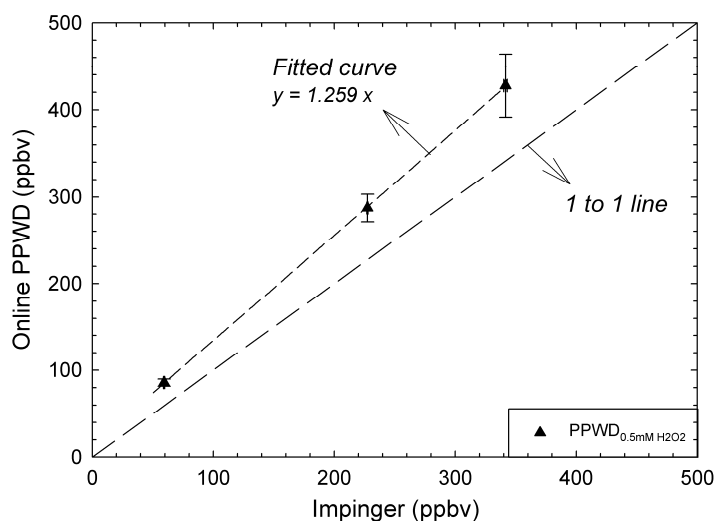
Fig. 8. Comparison of acetic acid gas concentrations determined by the impinger and by the online PPWD. The denuder liquid was 0.5 mM H 2 O 2 . The error bar represents one standard deviation.
