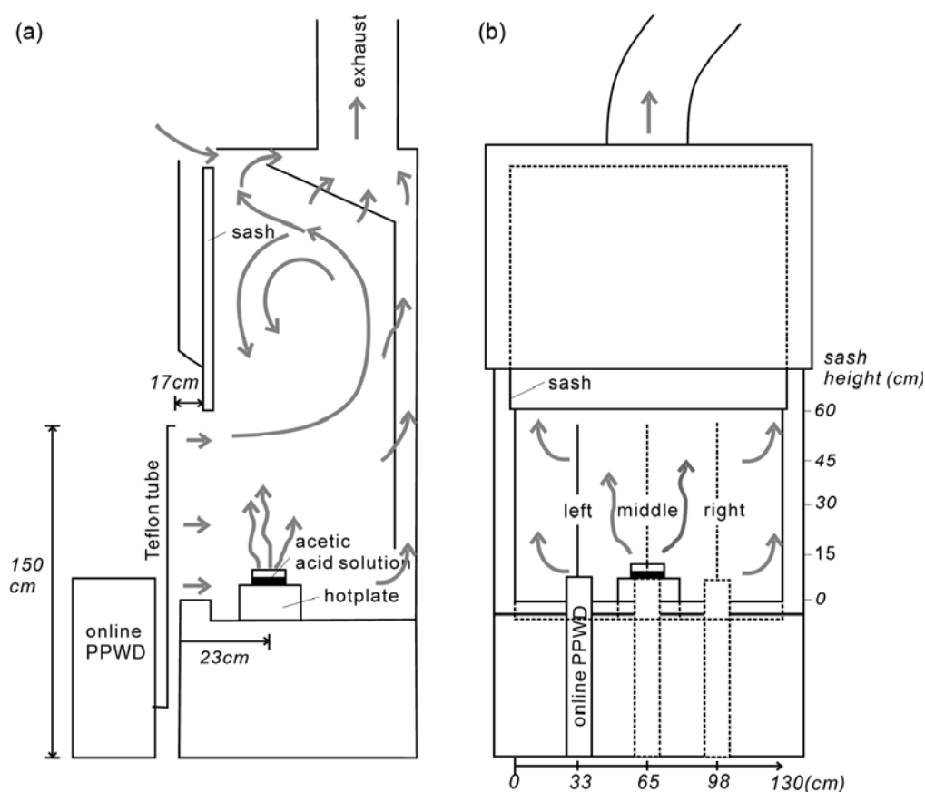
Fig. 6. Laboratory flume hood and experimental setup for exposure measurement of acetic acid gas (a) side view and (b) front view.
