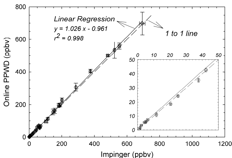
Fig. 7. Comparison of acetic acid gas concentration determined by the impinger with that determined by the online PPWD. Ultrapure water was the denuder liquid. The error bar represents one standard deviation.
