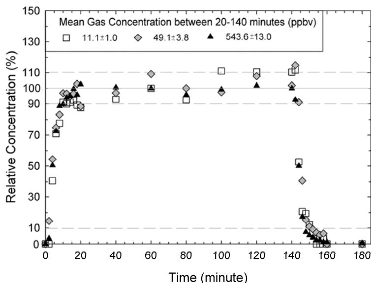
Fig. 10. Test results of response time for acetic acid gases of different concentrations. The x-axis represents the time of sampling.
