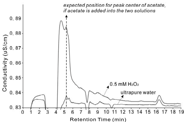
Fig. 9. Chromatograms of the two liquids: 0.5 mM H 2 O 2 and ultrapure water.
