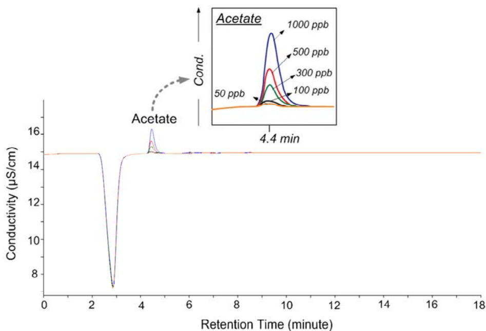
Fig. 2. Representative chromatogram.
