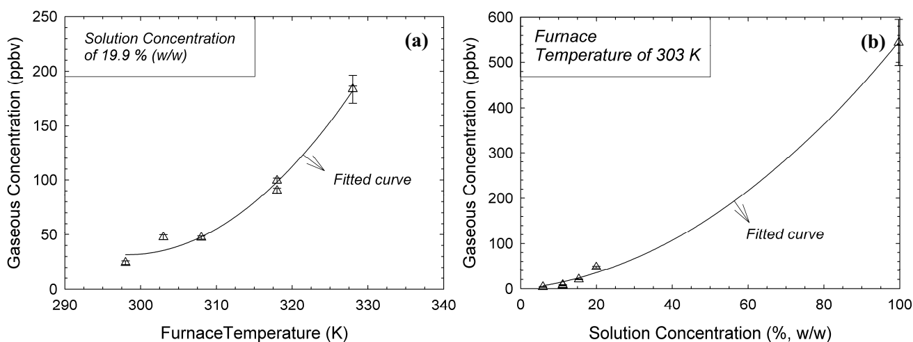
Fig. 4. Characteristics of test acetic acid gas generated from the evaporation tube depend on (a) furnace temperature and (b) aqueous solution concentration. Dilution and carrier gas flow rates were, respectively, fixed at 7920 and 80 cc/min. The error bar represents one standard deviation.
