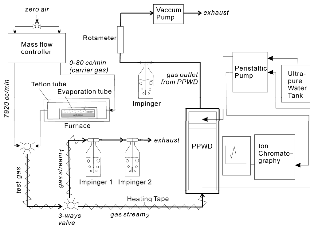
Fig. 3. Test setup: schematic diagram.
