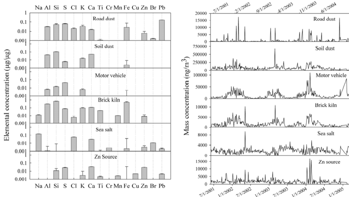
Fig. 1. Source composition profiles and time series of source contributions for coarse particulate matter.
