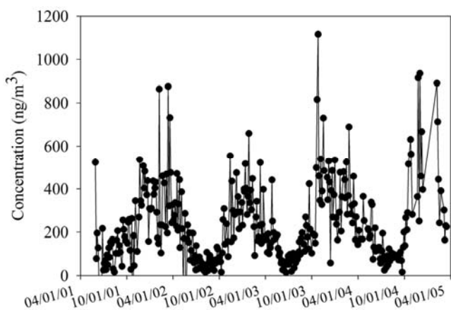
Fig. 5. Time series plot of the smoke contributions ( \text{ng/m}^3 ).
