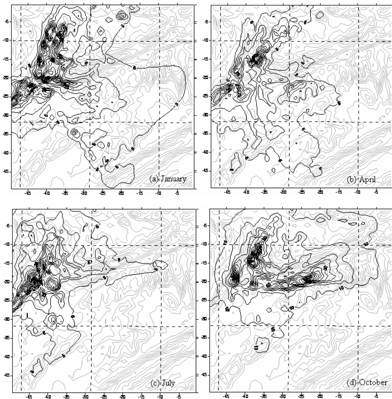
Fig. 4. (a-d) Monthly averaged SO 2 concentration increments ( \mu\text{g}/\text{m}^3 ) by elevated point source emissions in Chongqing in 2004. Gray background represents the terrain elevation.
