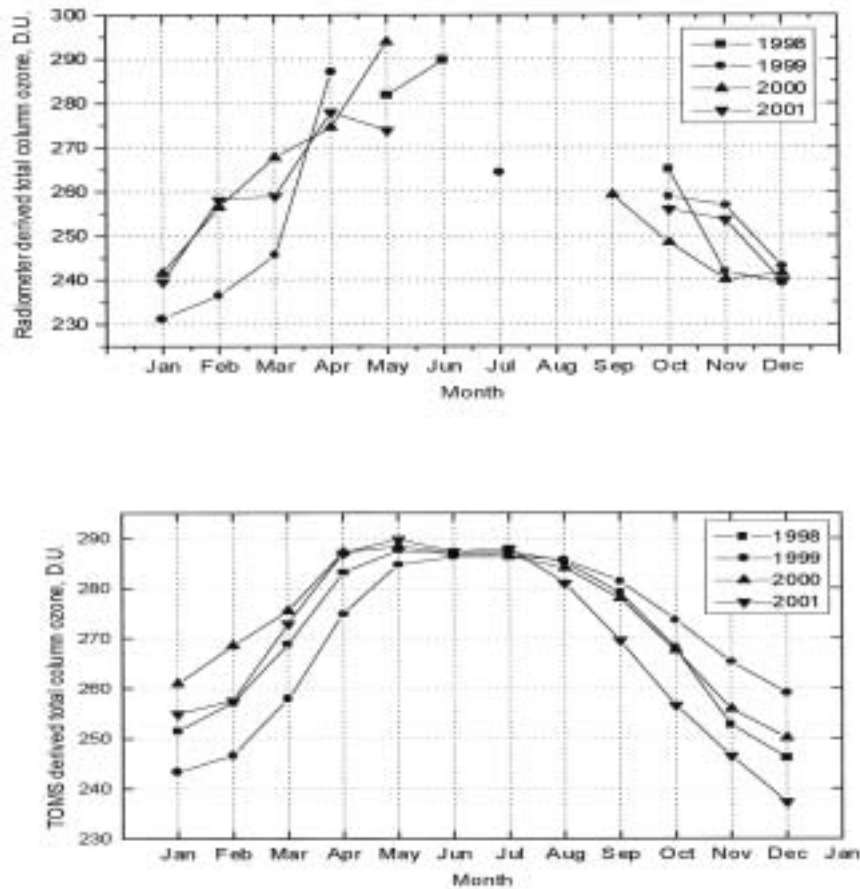
Figure 7. Comparison between total column ozone (TCO) measured by the ground-based (MICROTOPS II) radiometer and TOMS satellite over Pune during May 1998-December 2001.
