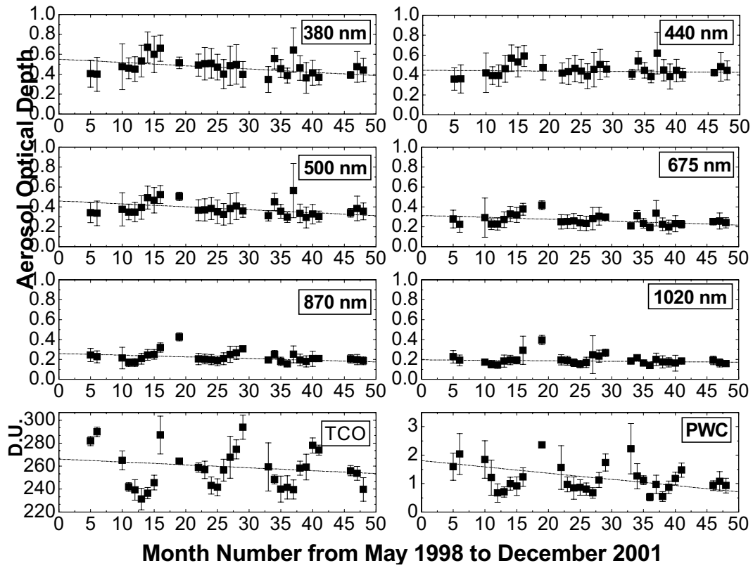
Figure 4. Long-term changes in monthly mean variations in AOD, TCO and PWC over Pune during May 1998-December 2001. The dashed line in each frame indicates trend line obtained from multiple regression analysis of data.
