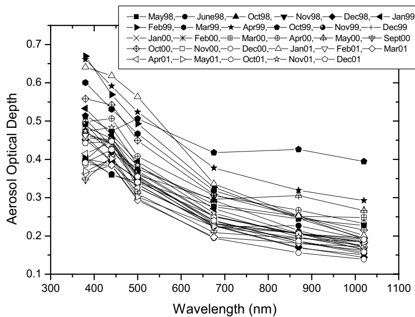
Figure 2. Monthly mean spectral distributions of AOD over Pune during May 1998-December 2001
