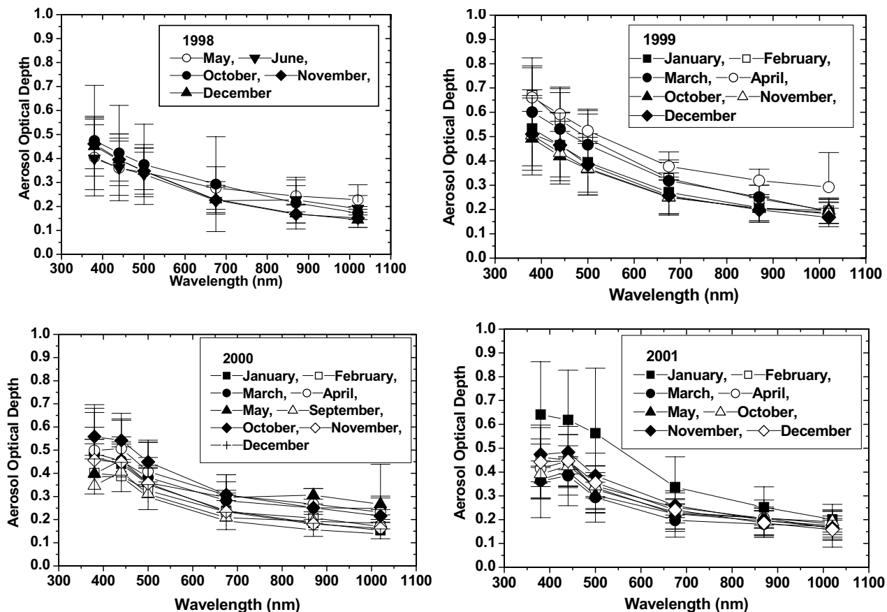
Figure 3. Wavelength dependence of aerosol optical depth during different months over Pune. Vertical lines at data points represent error bars.
