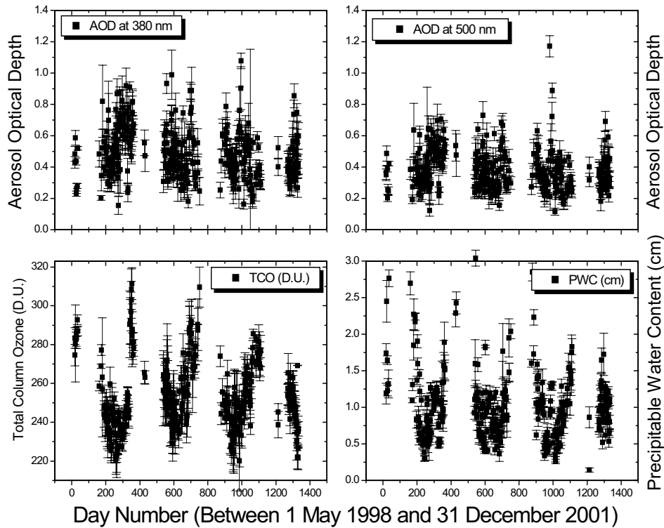
Figure 1. Daily mean variations in aerosol optical depth (AOD), total column ozone (TCO) and precipitable water content (PWC) over Pune during May 1998-December 2001. Vertical bars at each data point indicate positive and negative one sigma error.
