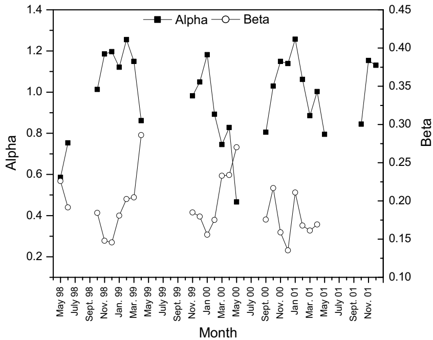
Figure 5. Monthly mean variations in Angstrom Coefficient (Beta) and Exponent (Alpha) observed over Pune during May 1998-December 2001.
